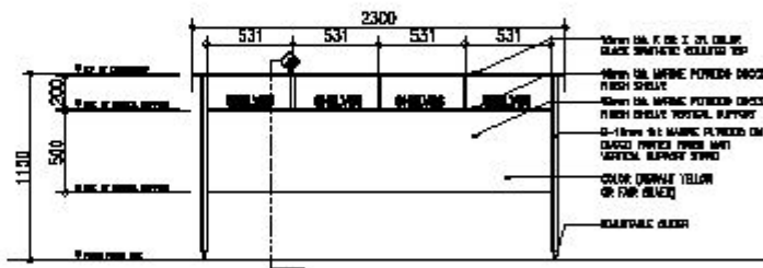
WRITING DECK FRONT ELEVATION SCALE: 1:20 METERS
